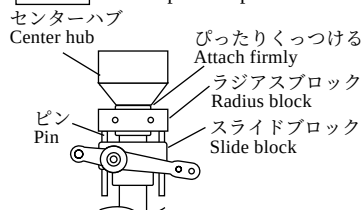
図-1 ピッチハイの時 Fig. 1 At full positive pitch
