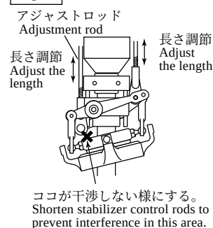
図-2 ピッチハイの時 Fig. 2 At full positive pitch
